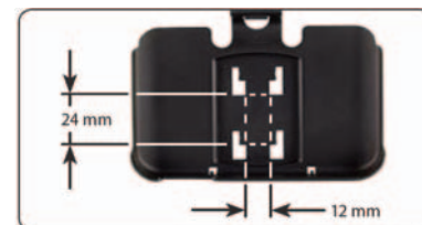
4-Prong Euro cradle (front) compatibility
