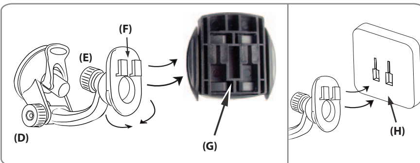
4-Prong Euro cradle (front) compatibility
